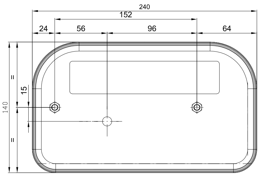
rear right lamp view FT-170 P - with lead
