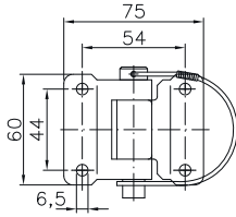
BSCH 30-5
